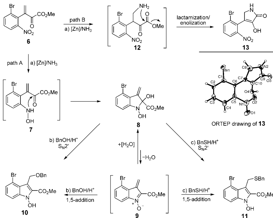
Scheme 3. Zn/ \text{NH}_4\text{Cl} -induced generation and trapping of \alpha,\beta -unsaturated nitron 9 to form N -hydroxyindoles. Reagents and conditions: a) Zn dust (4.9 equiv), \text{BrCH}_2\text{CH}_2\text{Br} (0.33 equiv), THF, reflux, 1 h; then cool to 25°C; then TMSCl (0.2 equiv); and then a mixture of aqueous \text{NH}_4\text{Cl} (1.0 N; 2.2 equiv) and 6 (1.0 equiv), 25°C, 15 min, 8 (56%), 13 (10%); b) 8 (1.0 equiv), p TsOH (3.0 equiv), molecular sieves (4 Å; 20 wt%), BnOH (5.0 equiv), DME, 40°C, 3 h, 10 (55%); c) 8 (1.0 equiv), p TsOH (3.0 equiv), molecular sieves (4 Å; 20 wt%), BnSH (5.0 equiv), DME, 40°C, 1 h, 11 (90%). TMS = trimethylsilyl; p TsOH = p -toluenesulfonic acid; Bn = benzyl; DME = 1,2-dimethoxyethane. ORTEP drawing of 13 drawn at the 50% probability level.
