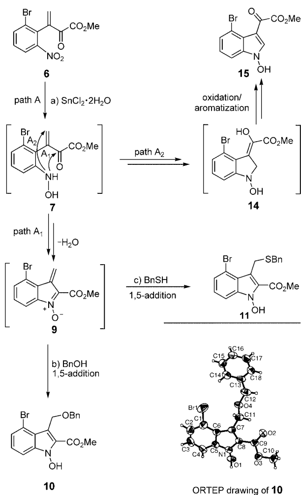
Scheme 4. \text{SnCl}_2 \cdot 2\text{H}_2\text{O} -induced generation and trapping of \alpha,\beta -unsaturated nitron 9 to form N -hydroxyindoles. Reagents and conditions: a, b) \text{SnCl}_2 \cdot 2\text{H}_2\text{O} (2.2 equiv), molecular sieves (4 Å; 20 wt%), BnOH (5.0 equiv), 6 (1.0 equiv), DME, 40 °C, 1.5 h, 10 (60%), 15 (17%); a, c) \text{SnCl}_2 \cdot 2\text{H}_2\text{O} (2.2 equiv), molecular sieves (4 Å; 20 wt%), BnSH (5.0 equiv), 6 (1.0 equiv), DME, 40 °C, 1 h, 11 (55%), 15 (15%). ORTEP drawing of 10 drawn at the 50% probability level.
