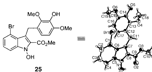
Figure 1. ORTEP drawing of compound 25 drawn at the 50% probability level.
